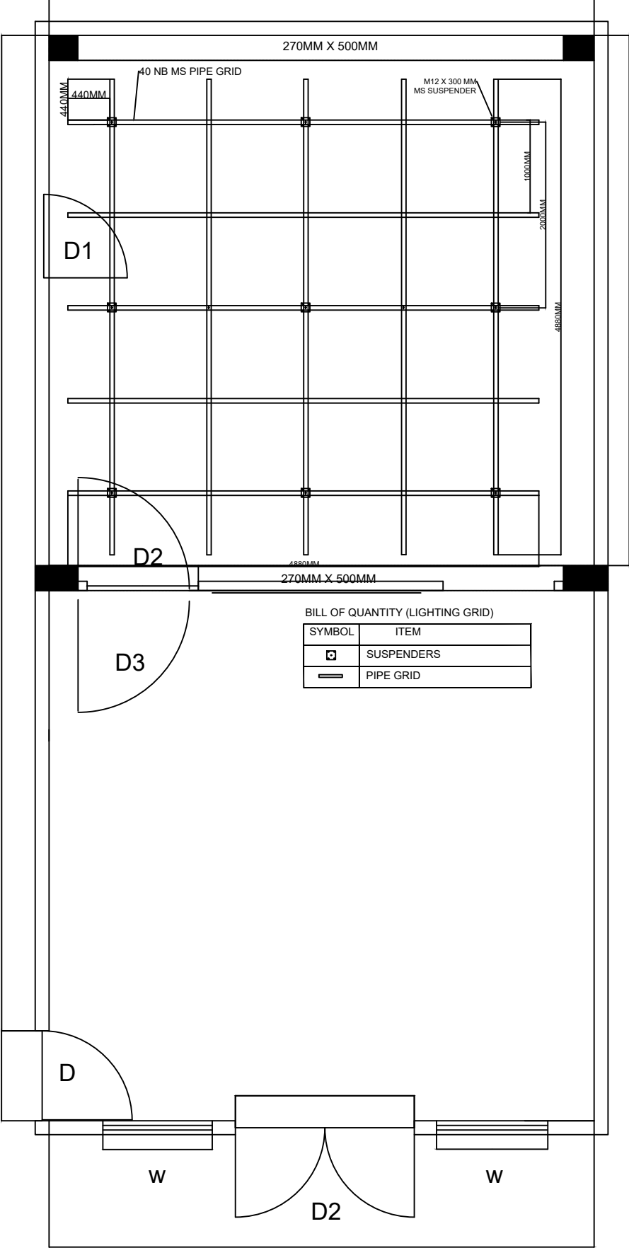
PIPE GRID LAYOUT
